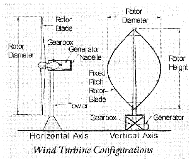
Figure 3 – Wind Turbine Configuration
